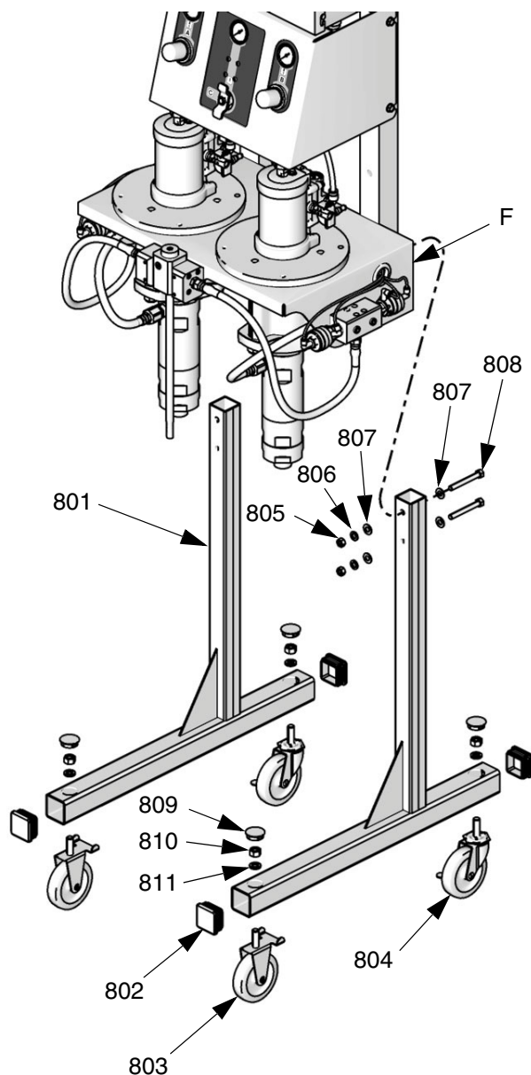
FIG. 1. 24F301 Stand Kit, for Pump-Based Systems
