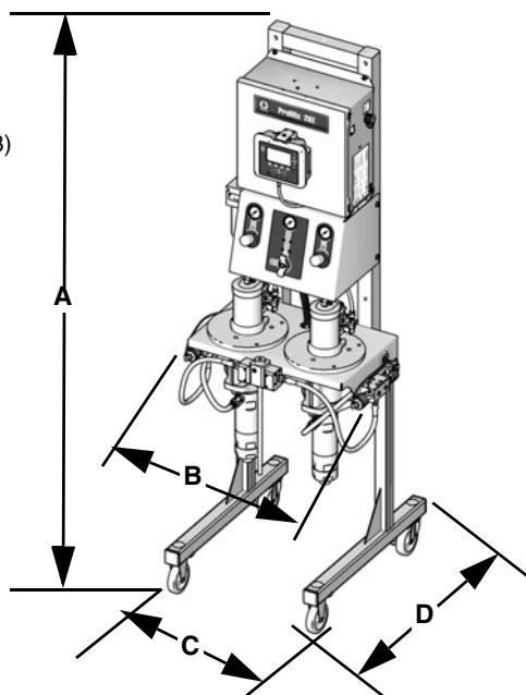
FIG. 1. 24F301 Stand Kit, for Pump-Based Systems
