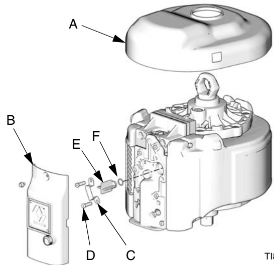
FIG. 2. Disassembly
